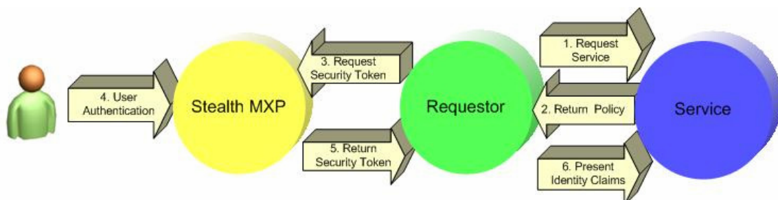
Figure 1: Security Token Flow with Stealth MXP
