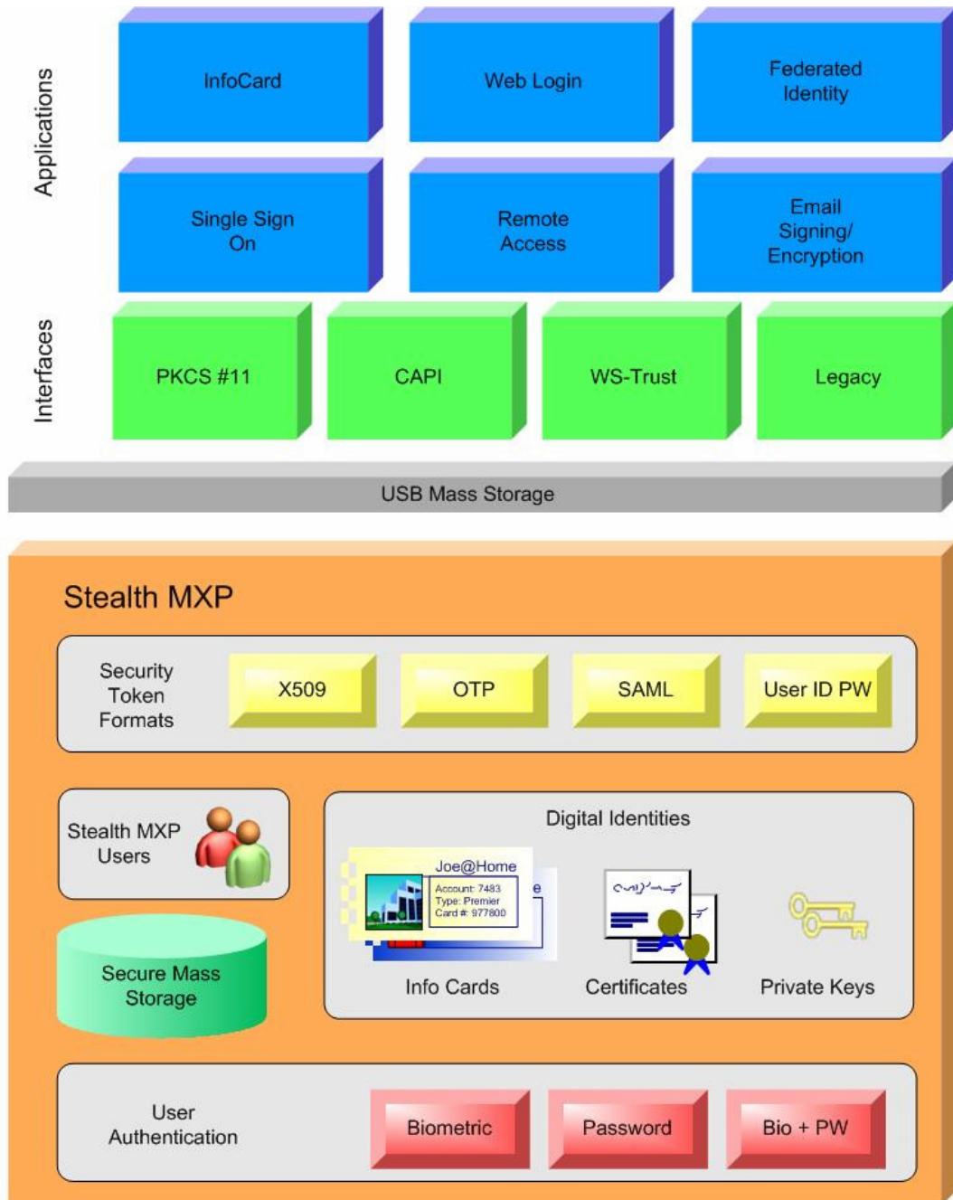
Figure 2: Stealth MXP and the Digital Identity Stack
